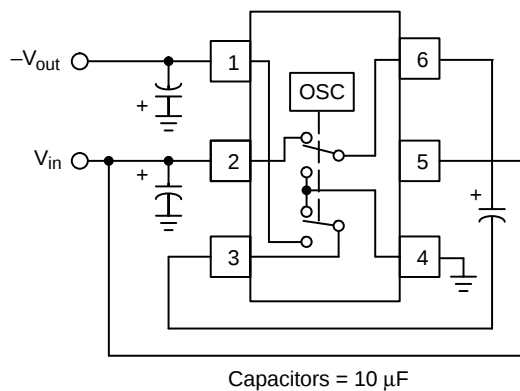
Figure 18. Voltage Inverter
