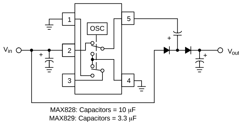
Figure 36. Positive Output Voltage Doubler
