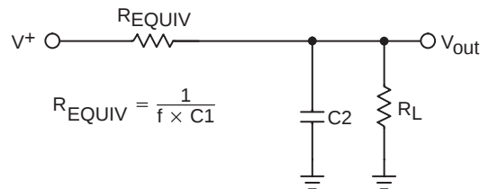
Figure 2b. Equivalent Output Resistance
