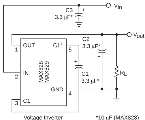
Figure 3. Test Circuit
