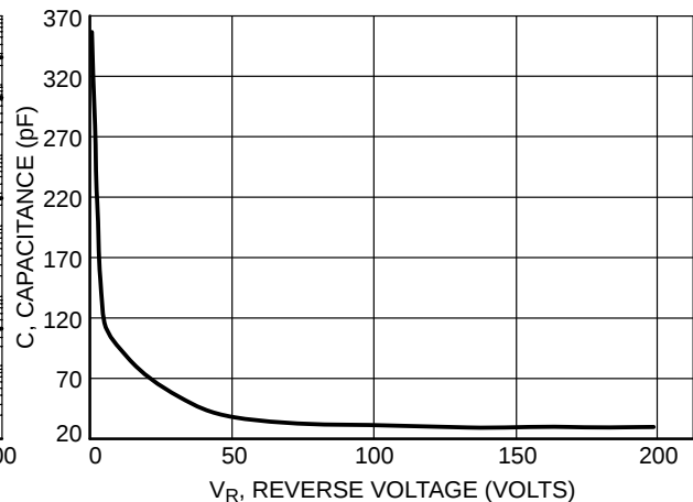
Figure 4. Typical Capacitance
