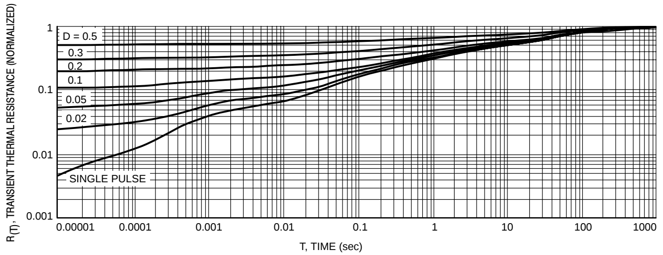
Figure 7. Thermal Resistance
