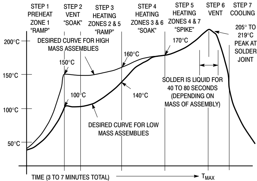
Figure 9. Typical Solder Heating Profile for D 2 PAK
