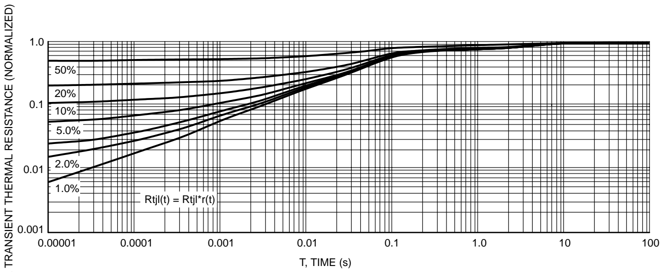
Figure 9. Thermal Response Junction to Lead
