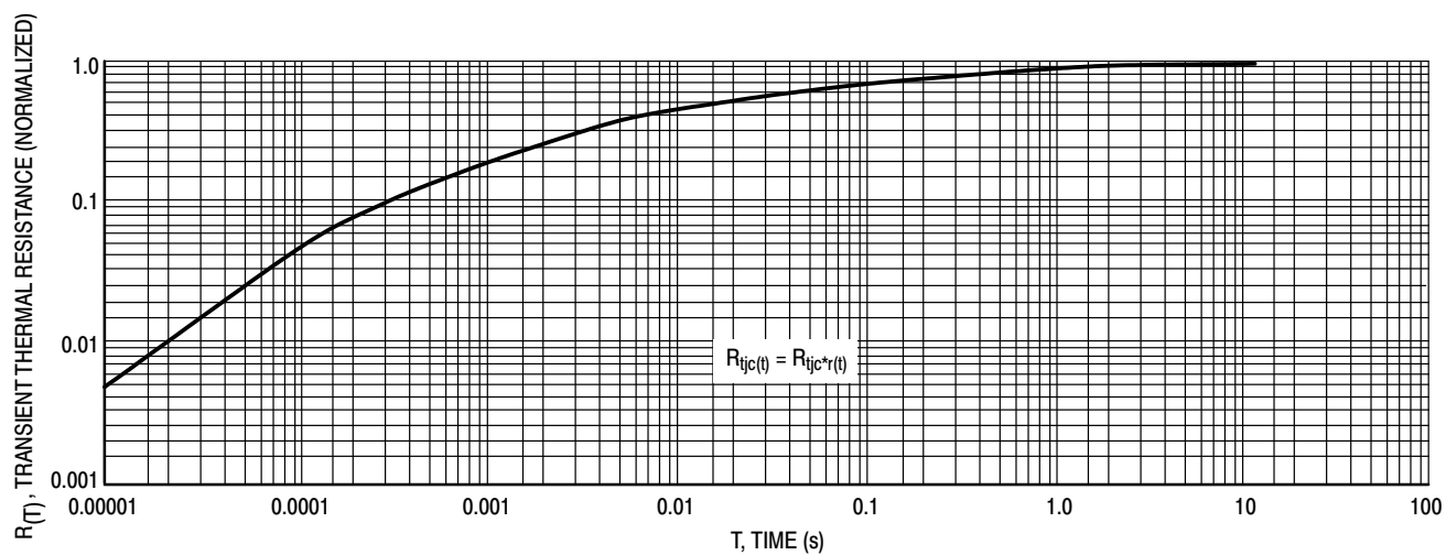
Figure 8. Thermal Response
