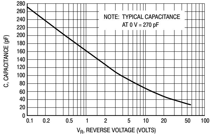
Figure 5. Typical Capacitance
