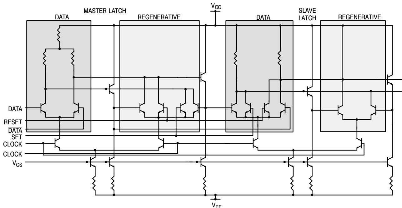
Figure 5. ECLinPS D Flip-Flop
