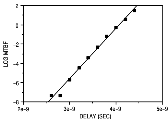
Figure 11. Plot of Log MTBF versus Delay
