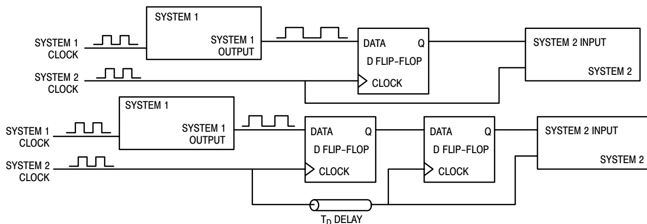
Figure 1. Clock Synchronization Schemes
