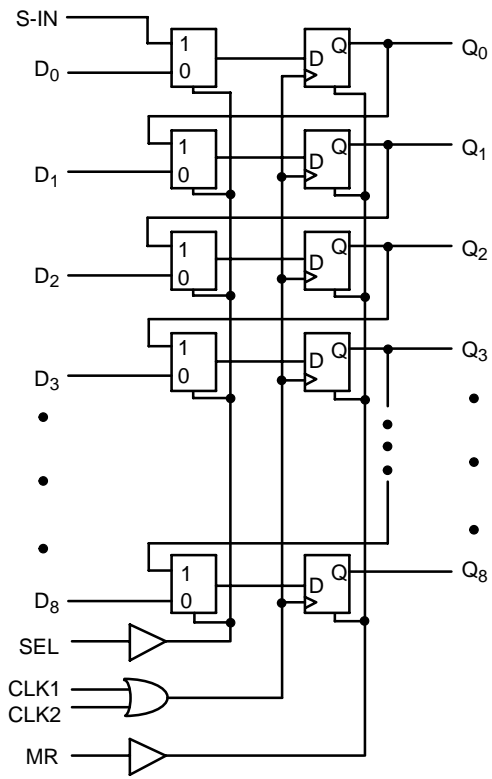
Figure 2. Logic Diagram
