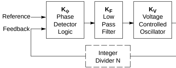
Figure 11. Fundamental Phase Lock Loop
