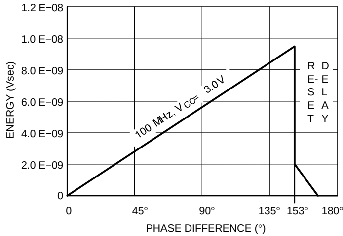
Figure 10. Typical U Output Pulse Energy vs. Phase Difference
