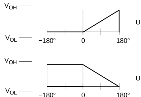
Figure 6. Average Output Voltage Levels for U and \bar{U} Outputs Per Phase Difference
