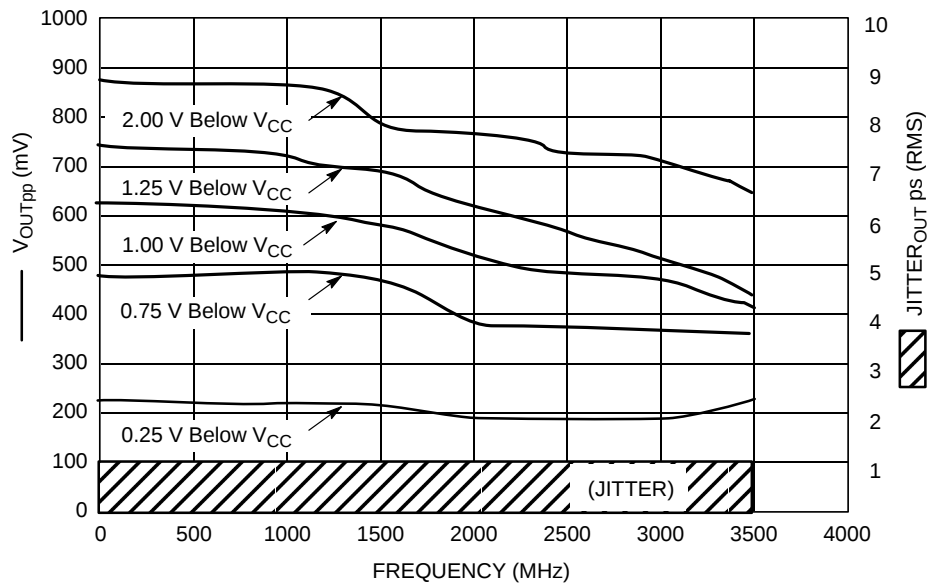
Figure 6. F_{max}/Jitter
