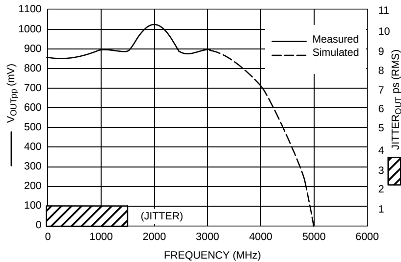
Figure 2. F_{\max}/\text{Jitter}
