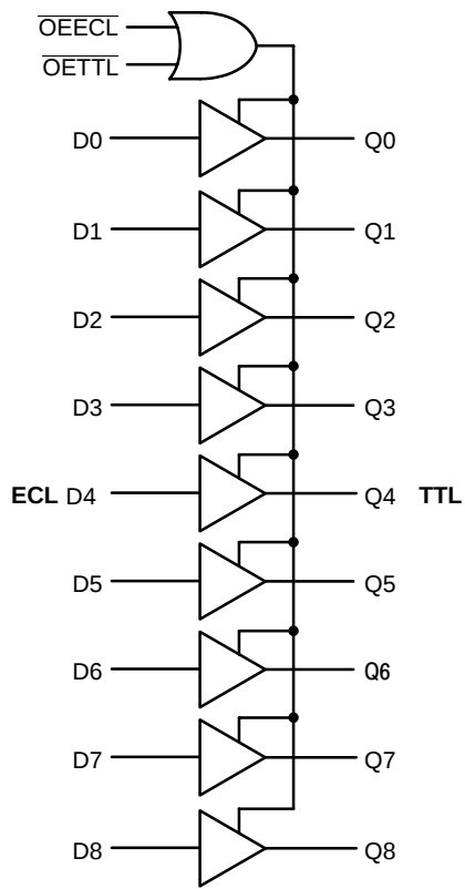
Figure 1. Logic Diagram
