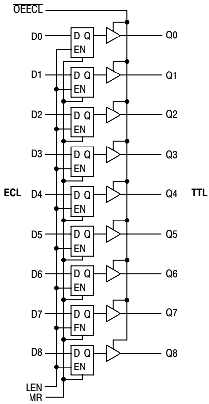
Figure 2. Logic Diagram
