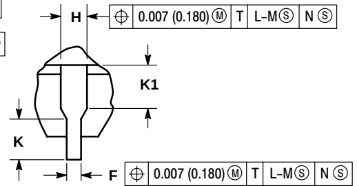
VIEW S
