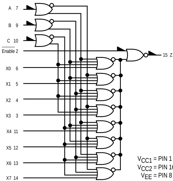
LOGIC DIAGRAM
