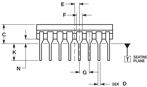
CDIP-16 L SUFFIX CERAMIC DIP PACKAGE CASE 620A-01 ISSUE O
