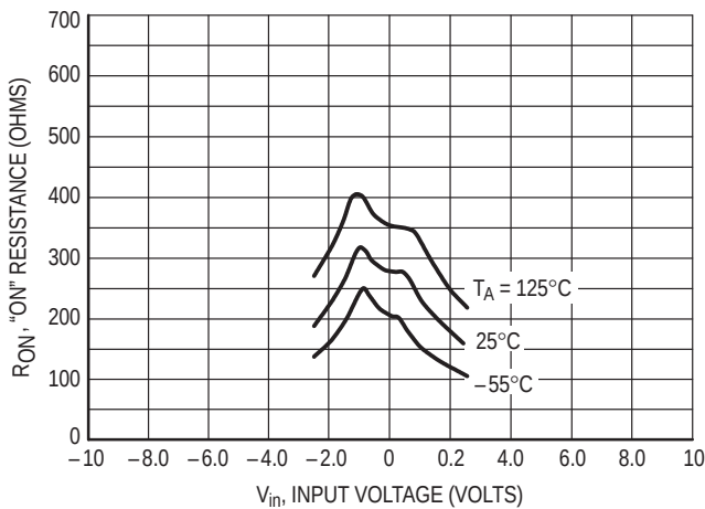
Figure 10. V_{DD} = 2.5 V, V_{SS} = -2.5 V
