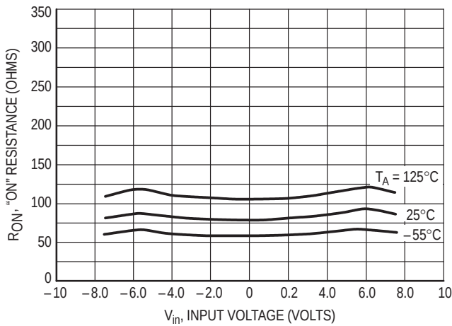
Figure 8. V_{DD} = 7.5 V, V_{SS} = -7.5 V
