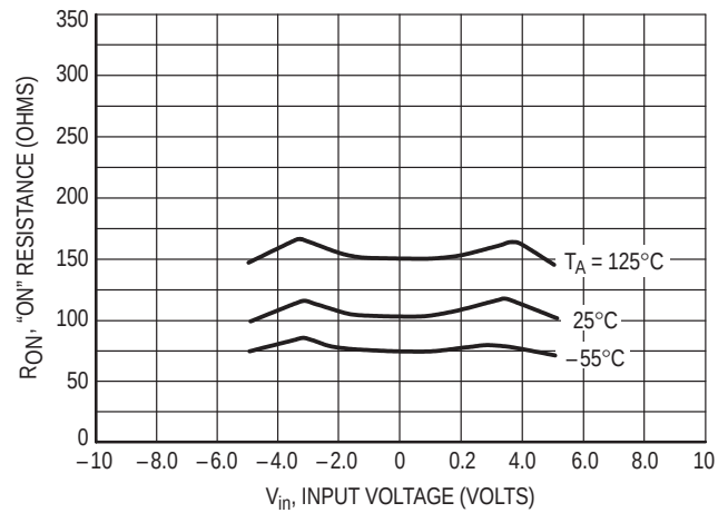
Figure 9. V_{DD} = 5.0 V, V_{SS} = -5.0 V
