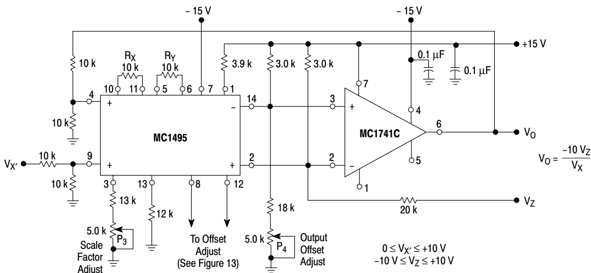
Figure 25. Divide Circuit
