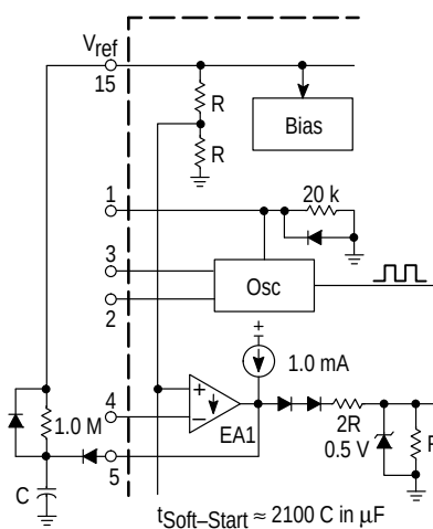
Figure 20. Soft-Start Circuit
