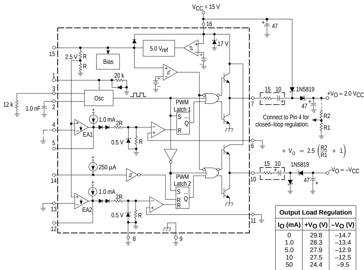
Figure 27. Dual Charge Pump Converter
