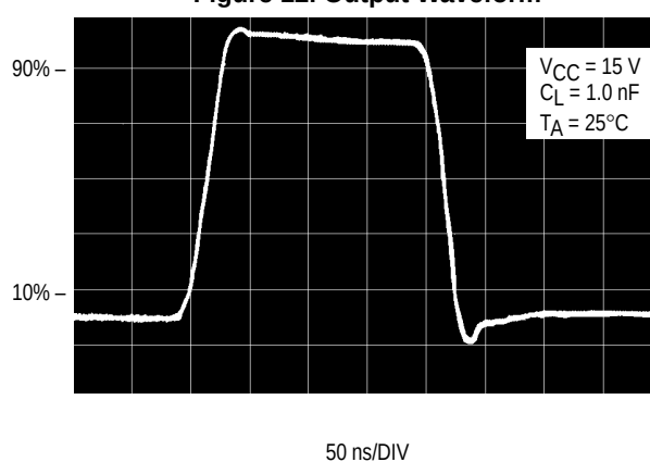
Figure 12. Output Waveform
