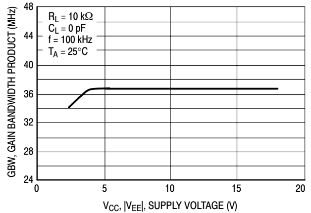
Figure 13. Gain Bandwidth Product versus Supply Voltage
