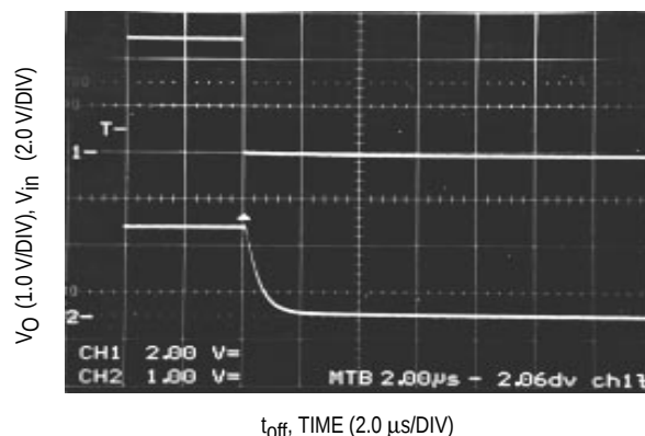
Figure 29. t_{off} Response
