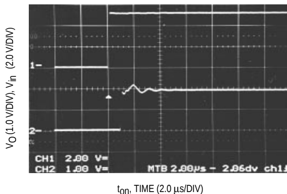
Figure 28. t_{on} Response
