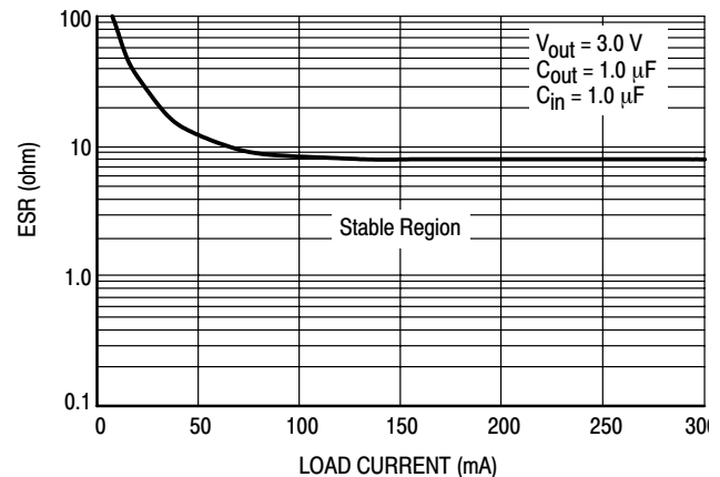
Figure 23. ESR for V_{\text{out}} = 3.0\text{V} Applications should be tested over all operating conditions to insure stability.
