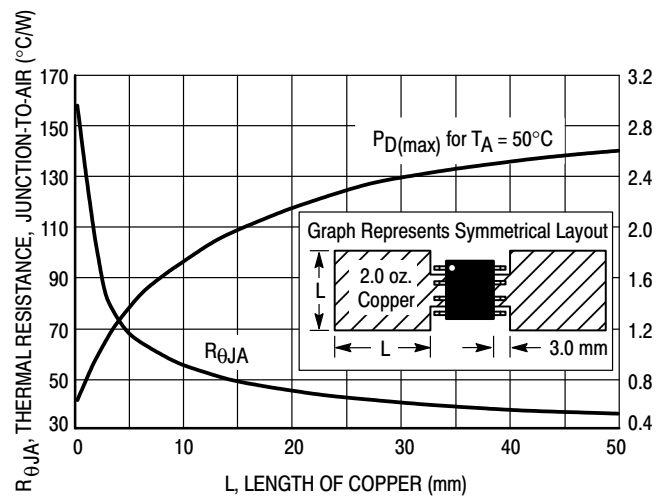
Figure 25. SOP-8 Thermal Resistance and Maximum Power Dissipation versus P.C.B. Copper Length
