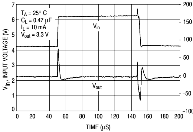
Figure 1. Line Transient Response
