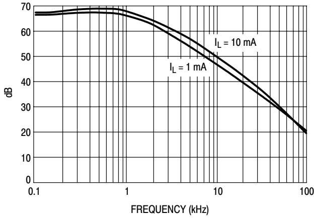
Figure 12. Ripple Rejection
