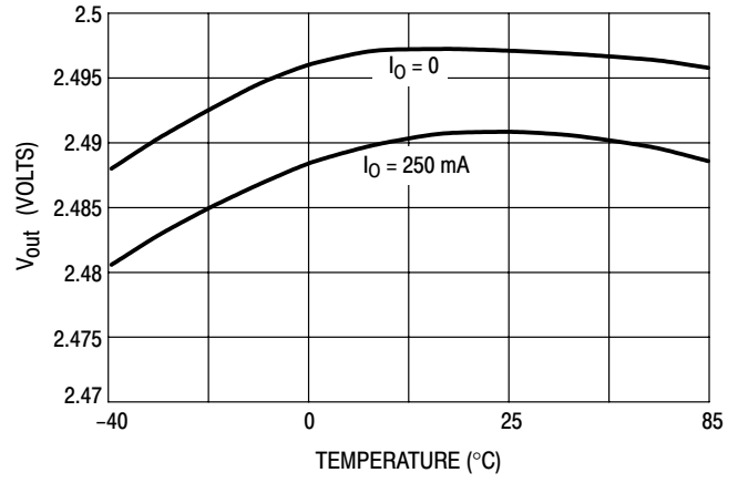
Figure 10. Output Voltage versus Ambient Temperature ( V_{in} = V_{out} + 1V )
