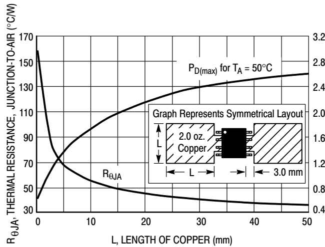
Figure 25. SOP-8 Thermal Resistance and Maximum Power Dissipation versus P.C.B. Copper Length
