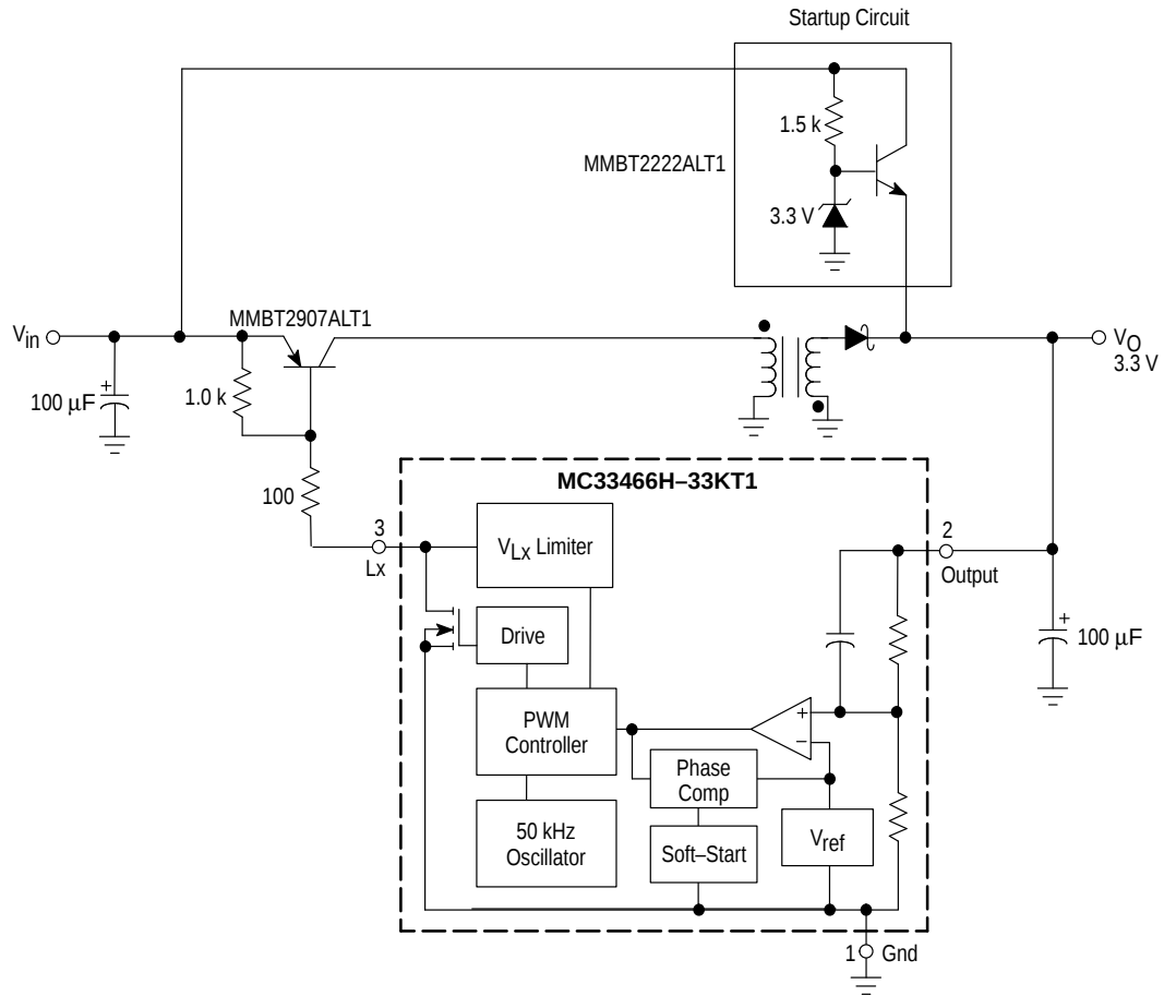
Figure 21. Flyback Application
