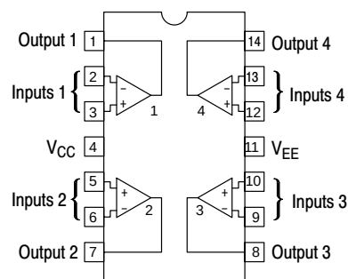
MC34004 (Top View)
