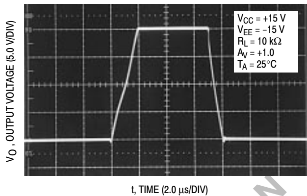
Figure 28. Transient Response
