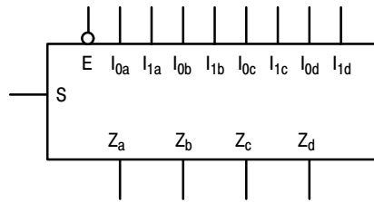
Figure 2. Logic Symbol
