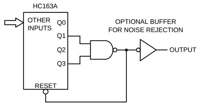
Figure 17. Modulo-11 Counter
