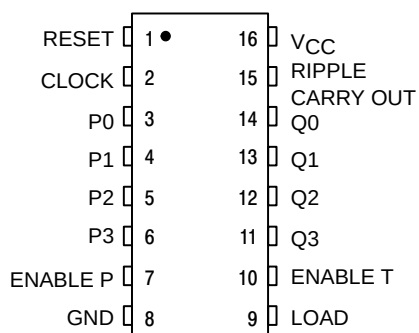
Figure 1. Pin Assignment
