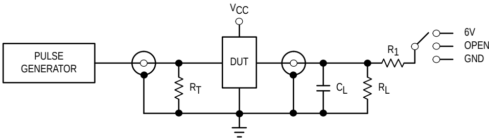
Figure 1. AC Waveforms
