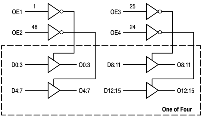
Figure 2. Logic Diagram
