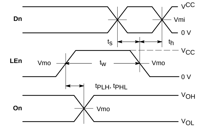
WAVEFORM 3 – LE to On PROPAGATION DELAYS, LE MINIMUM PULSE WIDTH, Dn to LE SETUP AND HOLD TIMES
