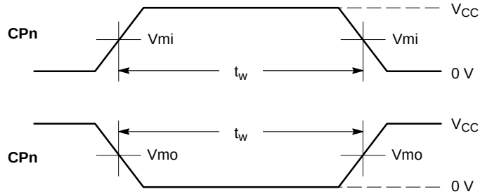
WAVEFORM 3 – PULSE WIDTH
