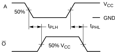
Figure 3. Switching Waveforms
