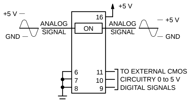
Figure 21. Application Example
