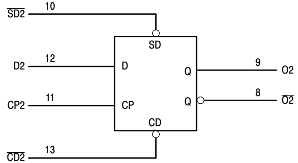
Figure 2. Logic Diagram
