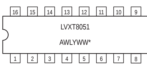
16-LEAD SOIC D SUFFIX CASE 751B
