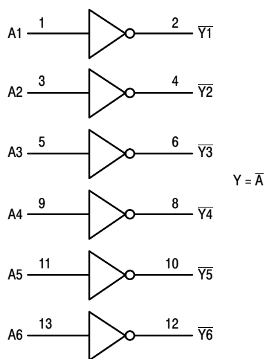
Figure 1. LOGIC DIAGRAM
