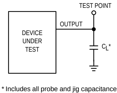
Figure 2. Test Circuit
