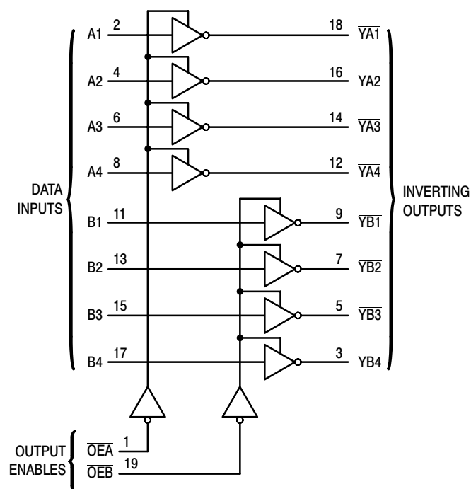
Figure 1. LOGIC DIAGRAM
