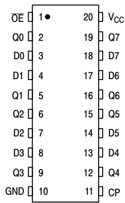
Figure 2. PIN ASSIGNMENT
