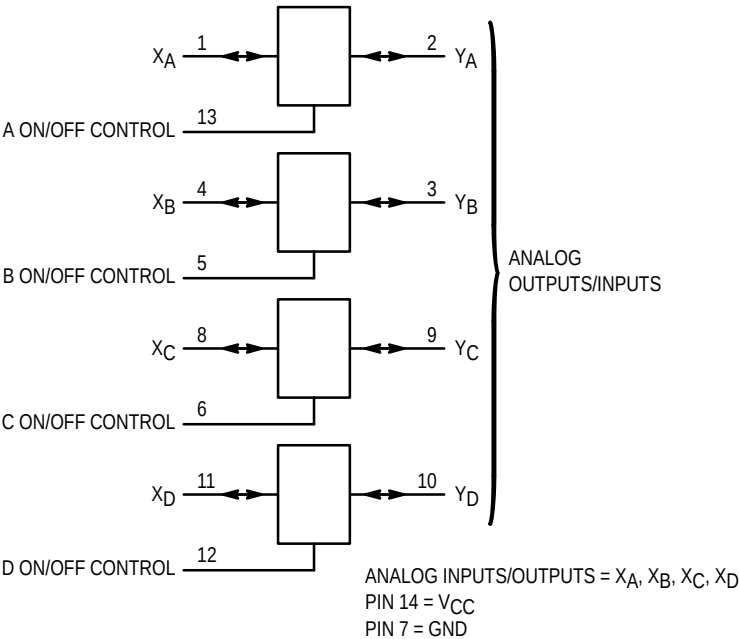
LOGIC DIAGRAM
