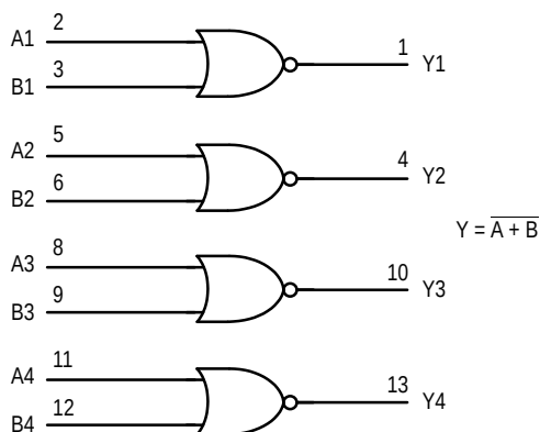
LOGIC DIAGRAM
