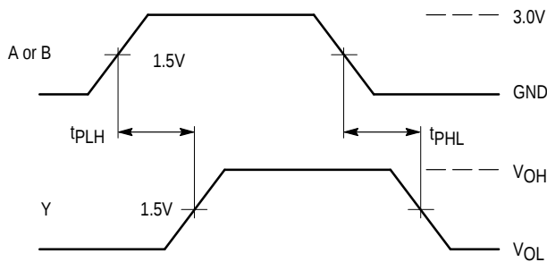
Figure 1. Switching Waveforms
