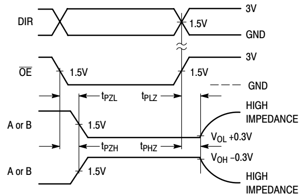
Figure 4. Switching Waveform
