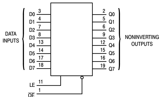
Figure 1. Logic Diagram
