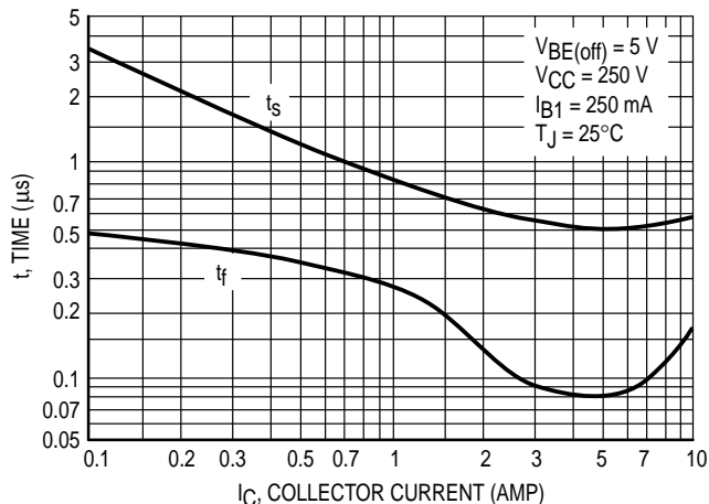
Figure 9. Turn-Off Time
