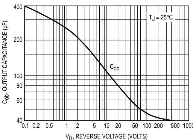
Figure 6. Output Capacitance
