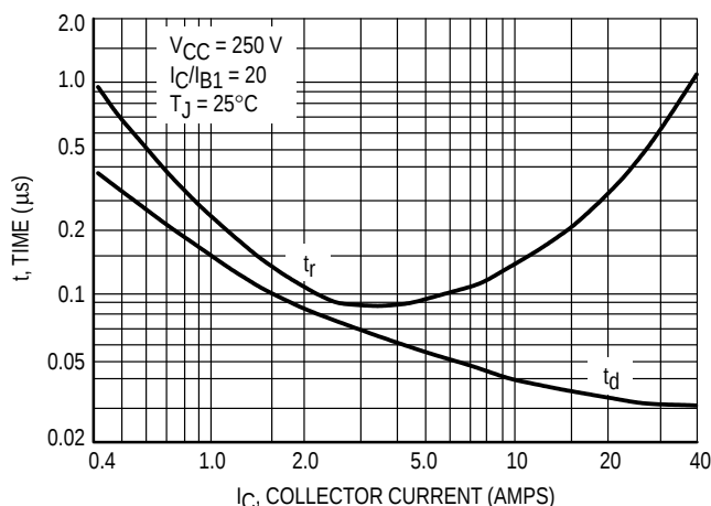
Figure 10. Typical Turn-On Switching Times
